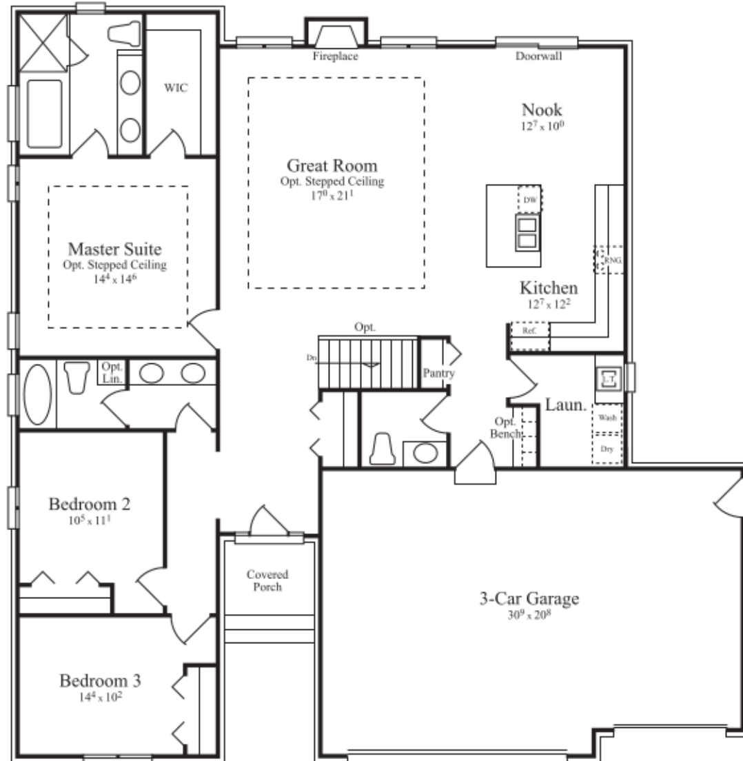
First Floor
